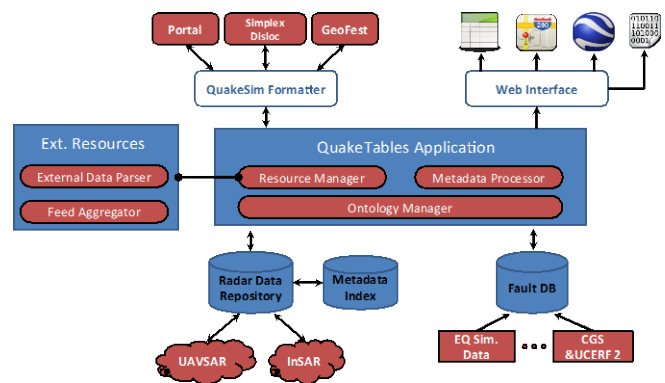
Figure 3. Quakesim QuakeTables architecture.
