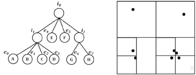
Figure 3 An example for SSP-Tree in 2D with 8 points
