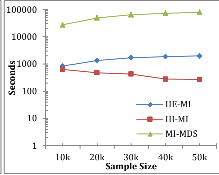
Figure 10 Execution time of three interpolation method
