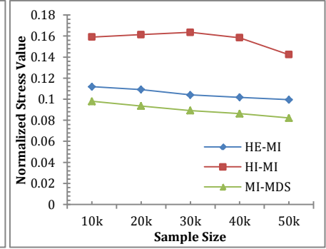
Figure 11 Normalized Stress value of 100k interpolation mapping result
