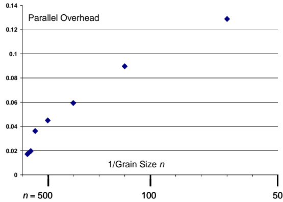
Figure 4. 8 core Parallel Overhead defined in Eq. (9) on Intel8b plotted against 8/N for GTM using M=256
